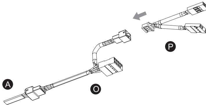
Connect the MB SYNC Cable to Water block
