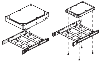
3.5" HDD
