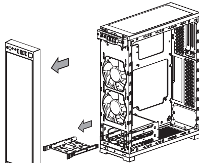
3.5" HDD
